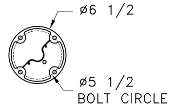
MOUNTING DETAIL
