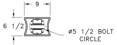
MOUNTING DETAIL
